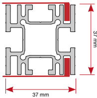
Fabric profile, half Total size: 37 x 37 x 3300 mm Weight: 3234 grams (980 g/m) Item IS-9330
