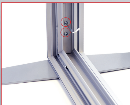
Lock the foot with the two screws.
